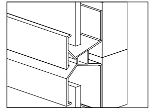
Horizontal joint profile
