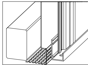
Starter profile foiled (vertical application only)
